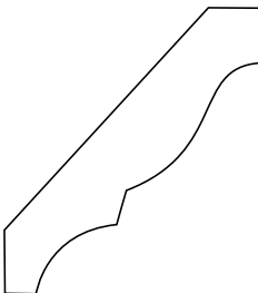
Panel Moulding 1" x 1 5/8"
