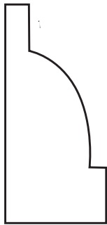
Rake Moulding 1 1/8" x 2 1/4"
